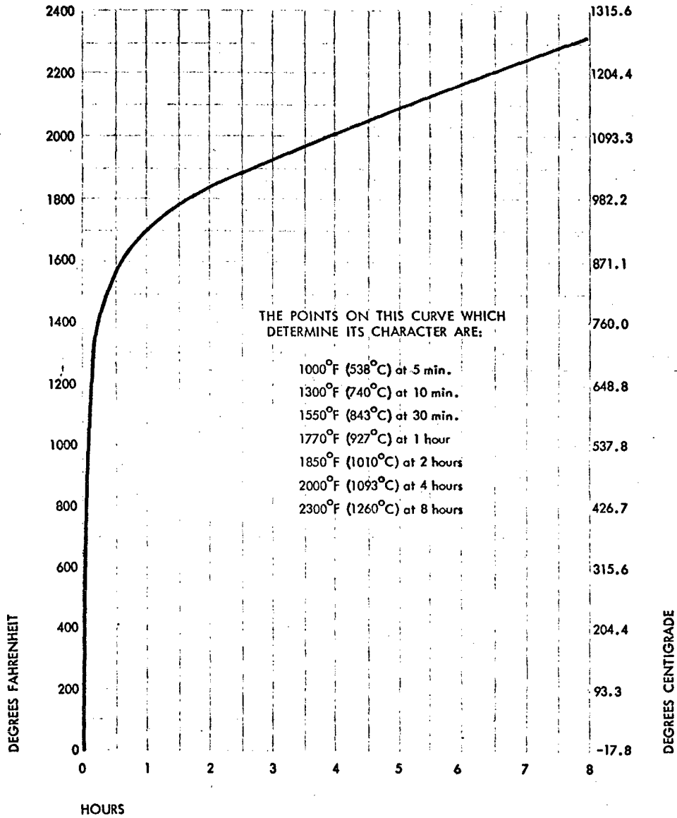
Figure D-1 STANDARD TIME-TEMPERATURE CURVE
